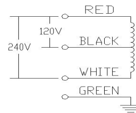
Connection Diagram
